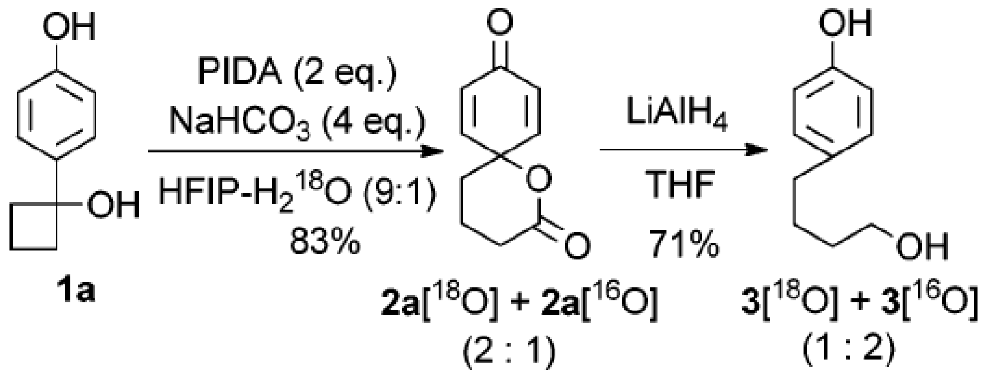
Scheme 4
