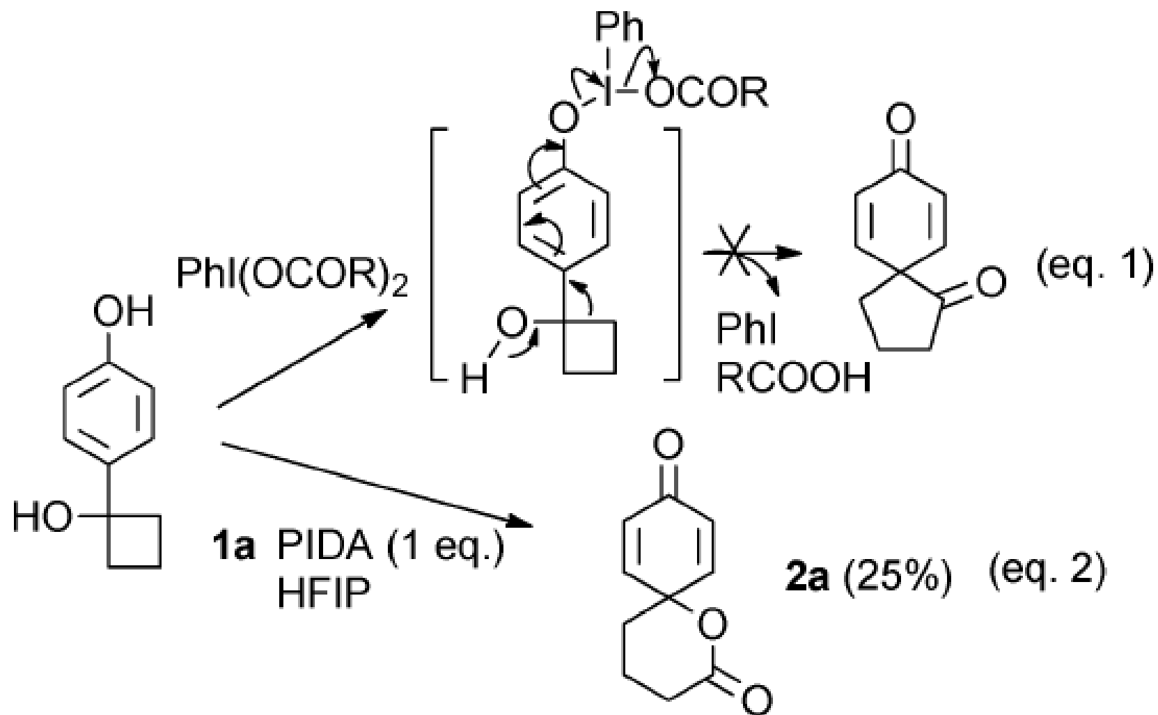
Scheme 2
