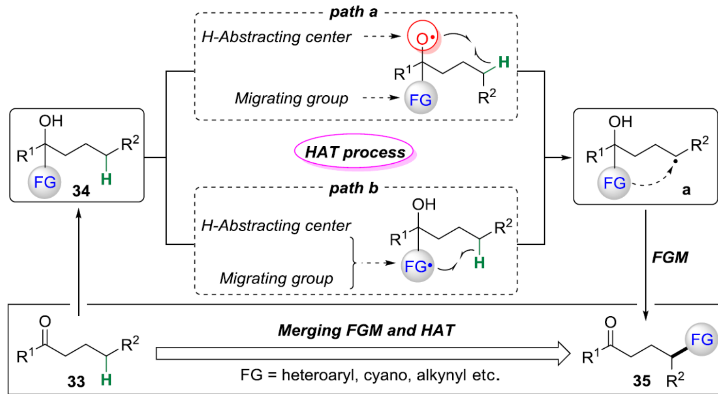
Scheme 24. C(sp 3 )-H Functionalization Strategy by Merging FGM and HAT
