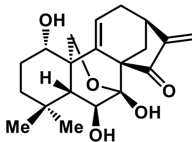
ericalyxin B (2)
