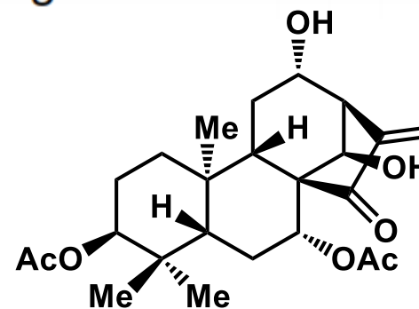
pharicin A (3)
