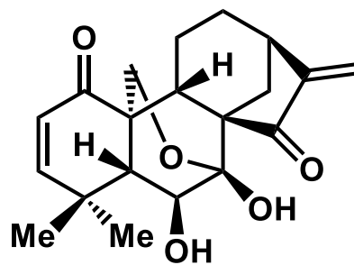
ericalyxin B (2)
