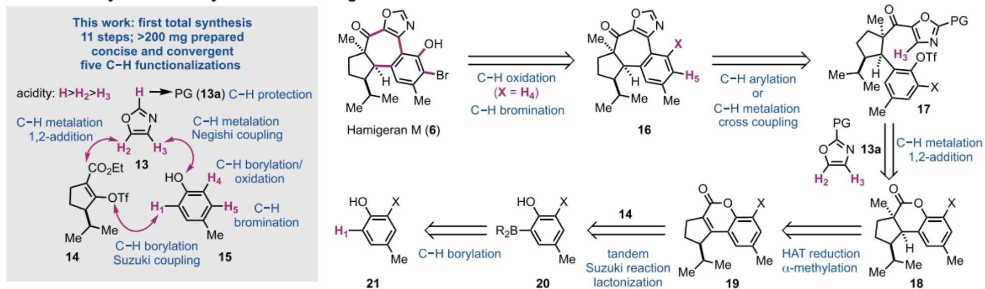
Figure 1. Hamigerans, plausible biosynthesis, and retrosynthetic analysis.
